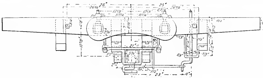
Fig. 2348. End Elevation.
